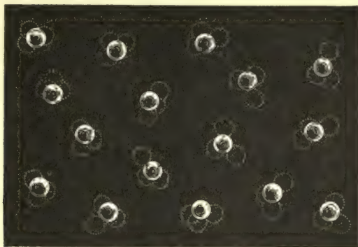
FIG. 33.—Brownian movement in milk. (According to O. Lehmann.)
